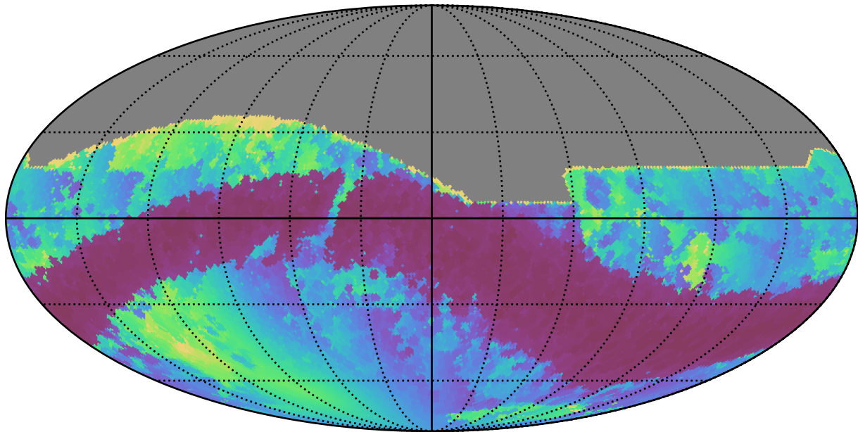
too_elab_r32_d2_giz_v3.4_10yrs All sky r band: Min solarElong
