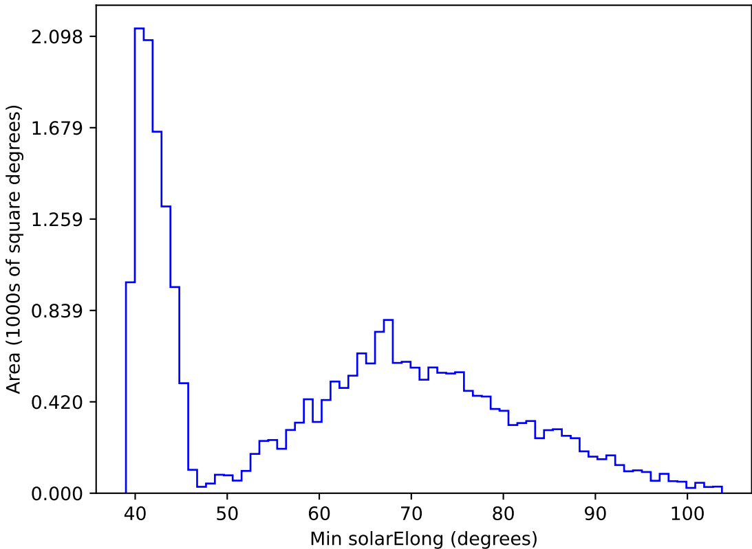
too_elab_r32_d2_giz_v3.4_10yrs All sky r band: Min solarElong
