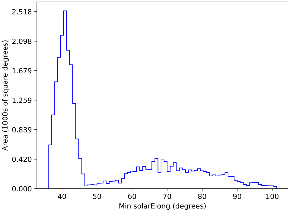
too_elab_r32_d2_giz_v3.4_10yrs All sky i band: Min solarElong
