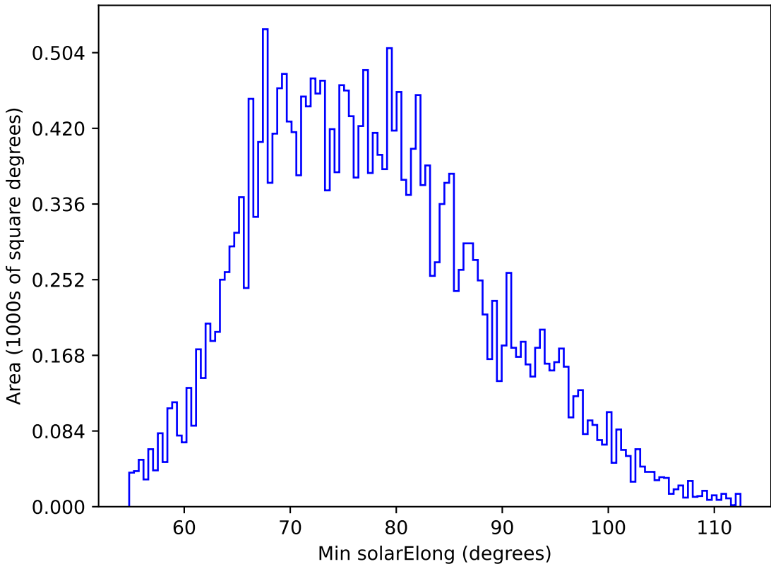
too_elab_r32_d2_giz_v3.4_10yrs All sky g band: Min solarElong
