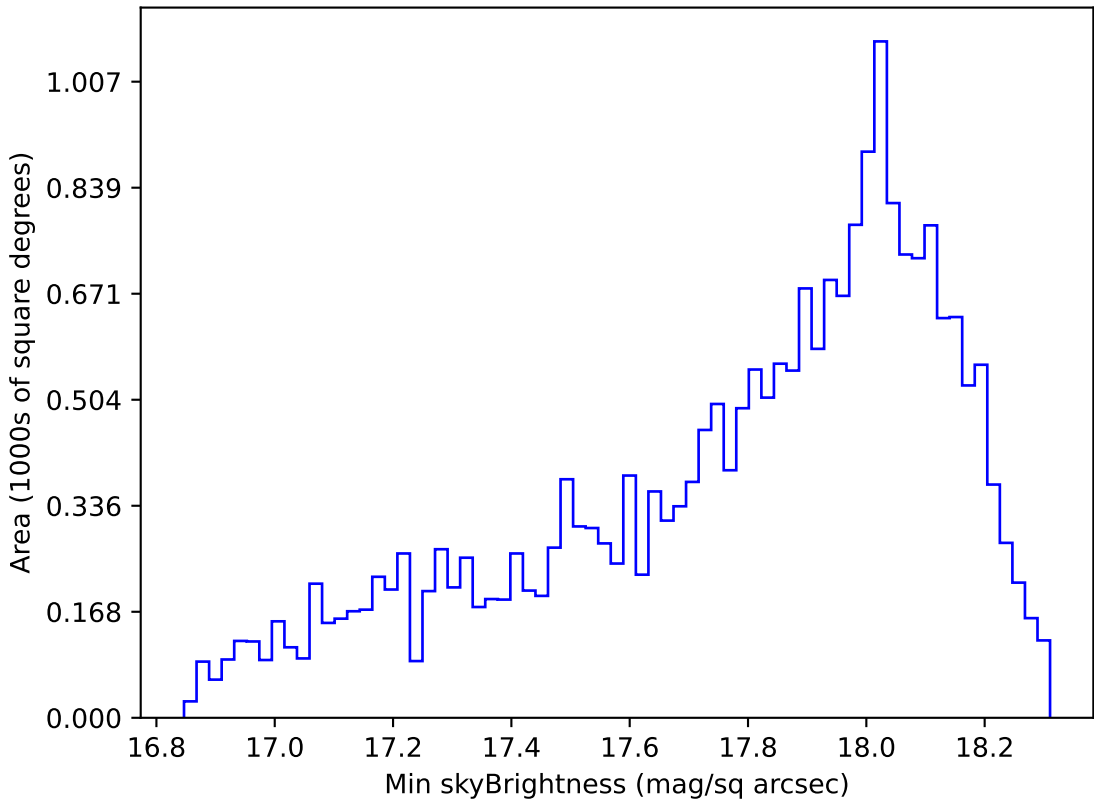
too_elab_r32_d2_giz_v3.4_10yrs Yr 1 y band: Min skyBrightness
