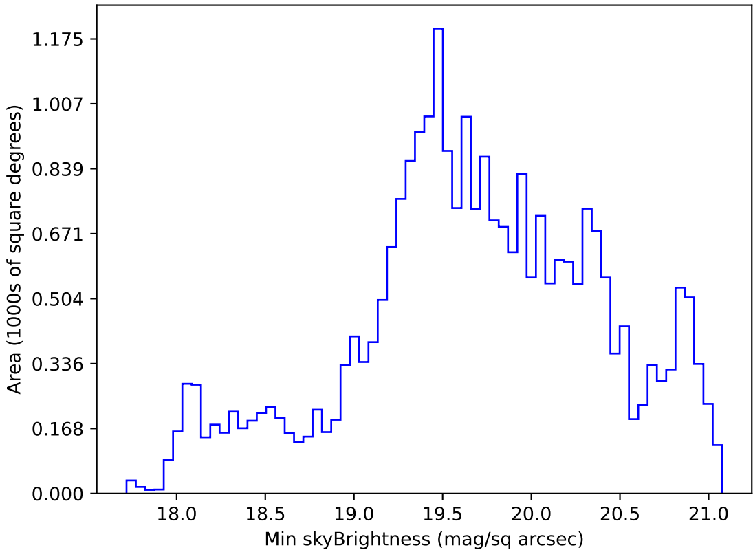
too_elab_r32_d2_giz_v3.4_10yrs Yr 1 r band: Min skyBrightness
