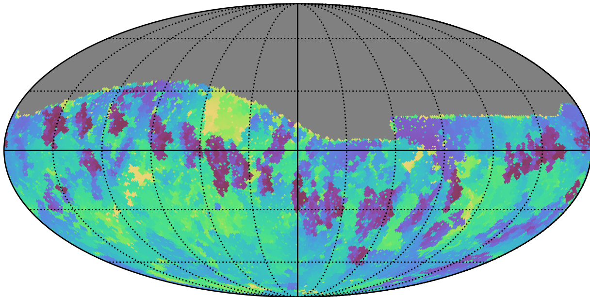
too_elab_r32_d2_giz_v3.4_10yrs Yr 1 i band: Min skyBrightness
