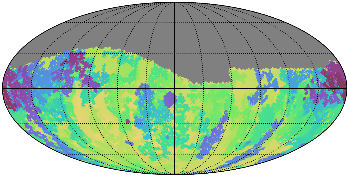
too_elab_r32_d2_giz_v3.4_10yrs Yr 1 g band: Min skyBrightness
