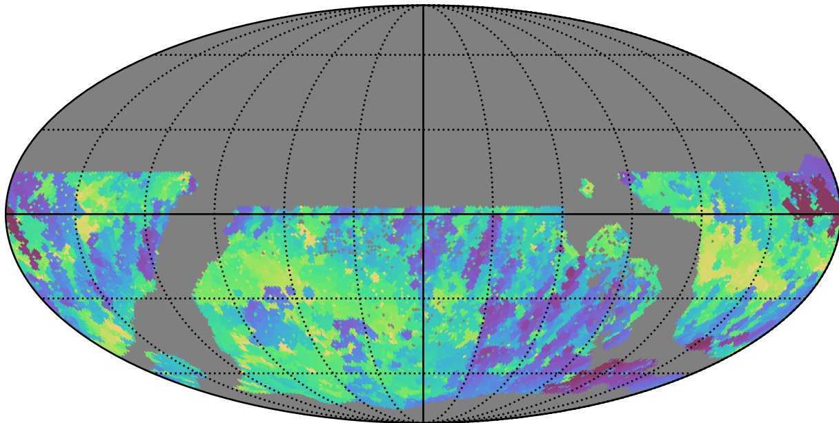
too_elab_r32_d2_giz_v3.4_10yrs WFD r band: Min skyBrightness
