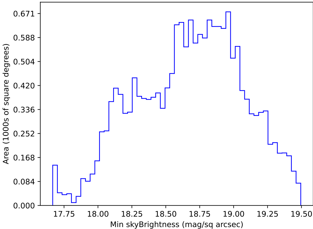
too_elab_r32_d2_giz_v3.4_10yrs WFD r band: Min skyBrightness
