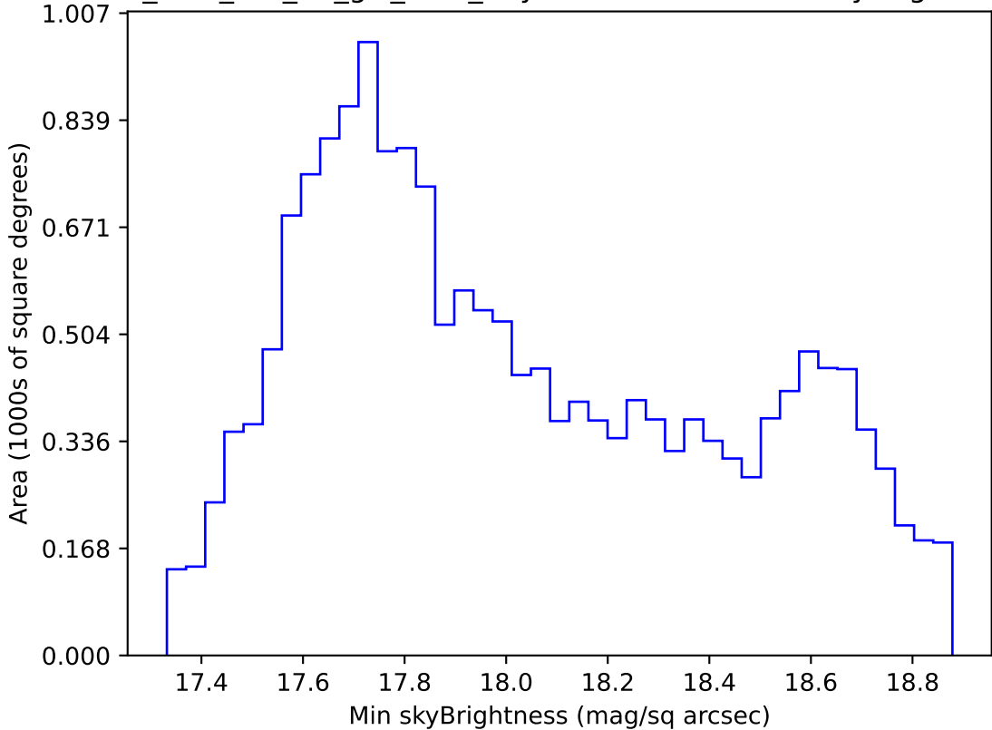
too_elab_r32_d2_giz_v3.4_10yrs WFD i band: Min skyBrightness
