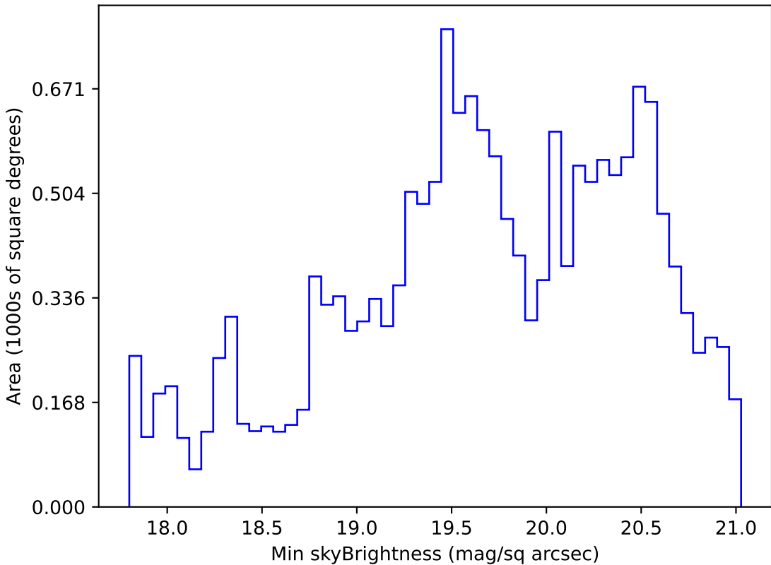
too_elab_r32_d2_giz_v3.4_10yrs WFD g band: Min skyBrightness
