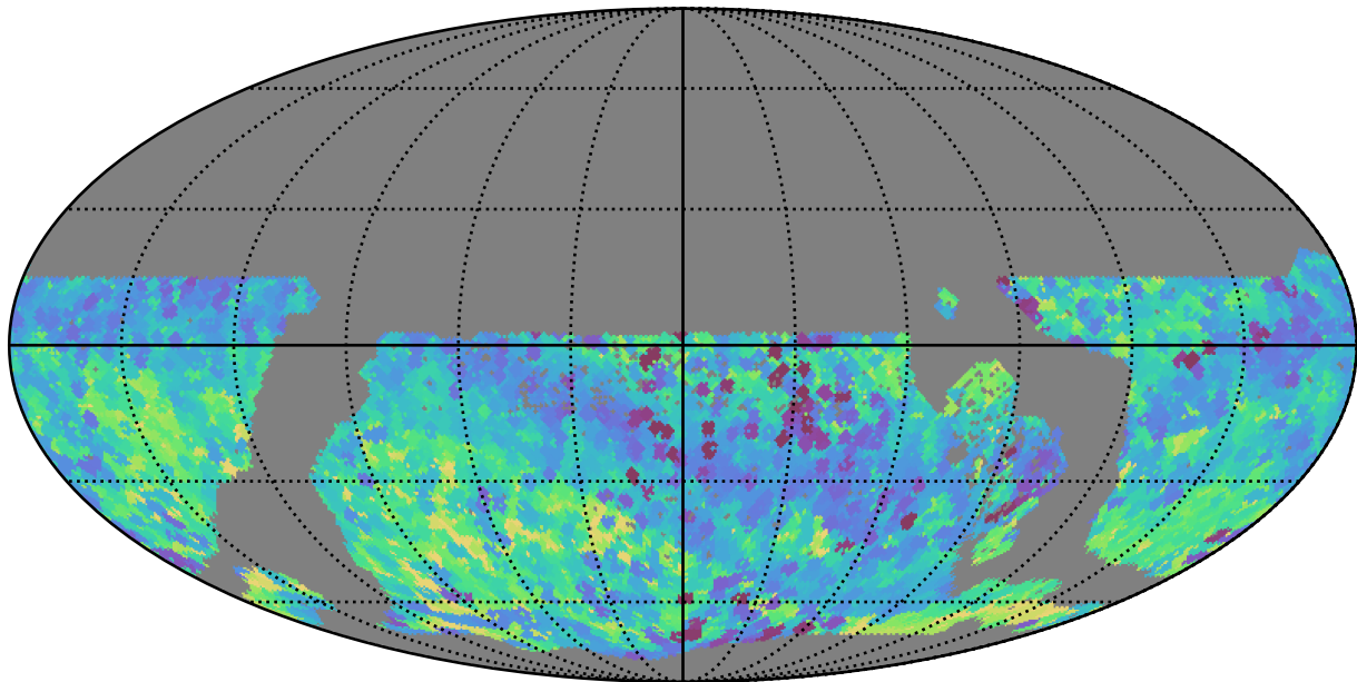
too_elab_r32_d2_giz_v3.4_10yrs WFD all bands: Min skyBrightness
