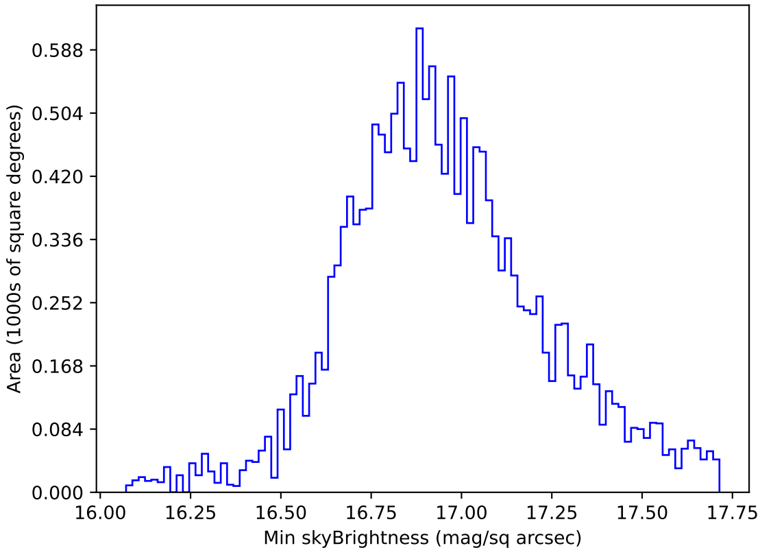
too_elab_r32_d2_giz_v3.4_10yrs WFD all bands: Min skyBrightness
