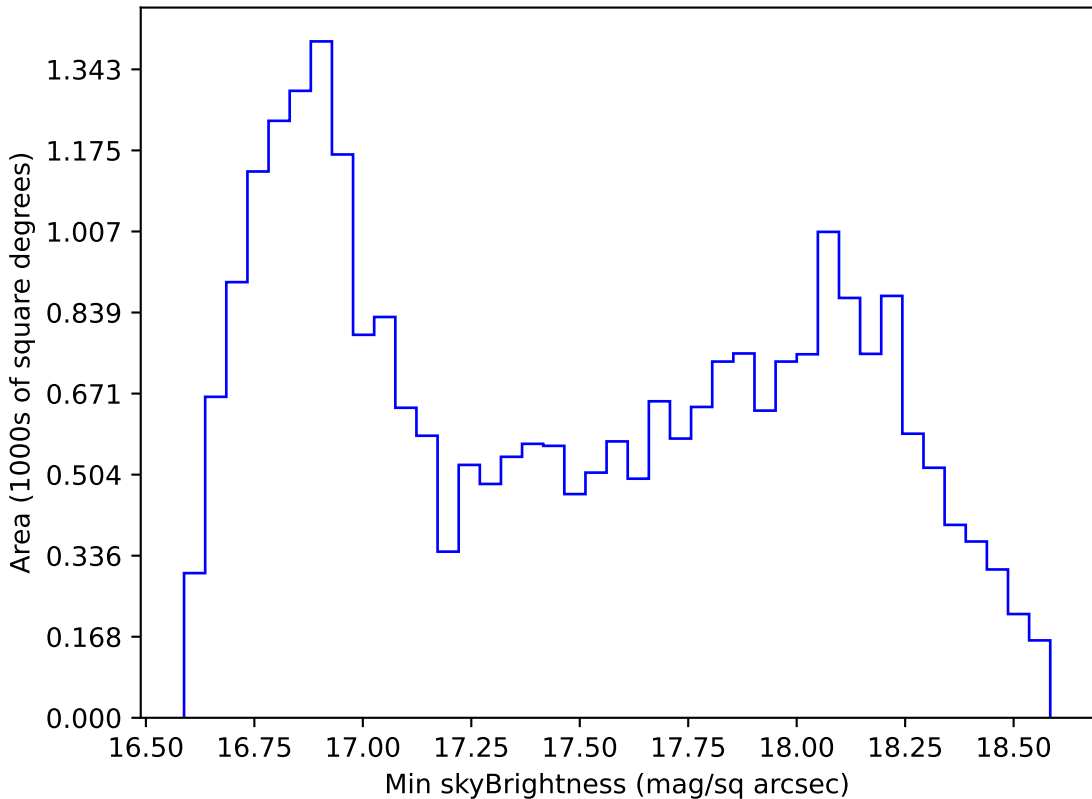
too_elab_r32_d2_giz_v3.4_10yrs All sky z band: Min skyBrightness
