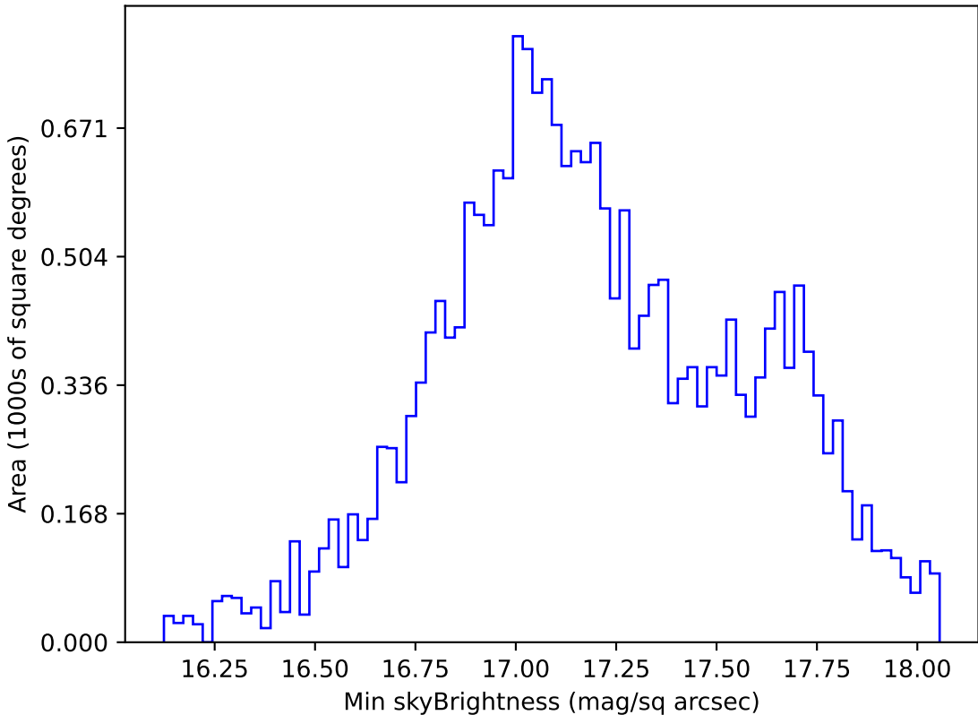
too_elab_r32_d2_giz_v3.4_10yrs All sky y band: Min skyBrightness
