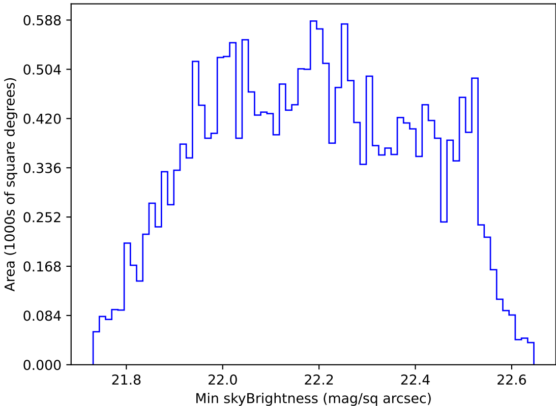
too_elab_r32_d2_giz_v3.4_10yrs All sky u band: Min skyBrightness
