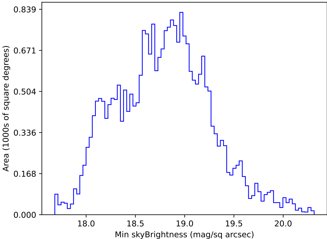
too_elab_r32_d2_giz_v3.4_10yrs All sky r band: Min skyBrightness
