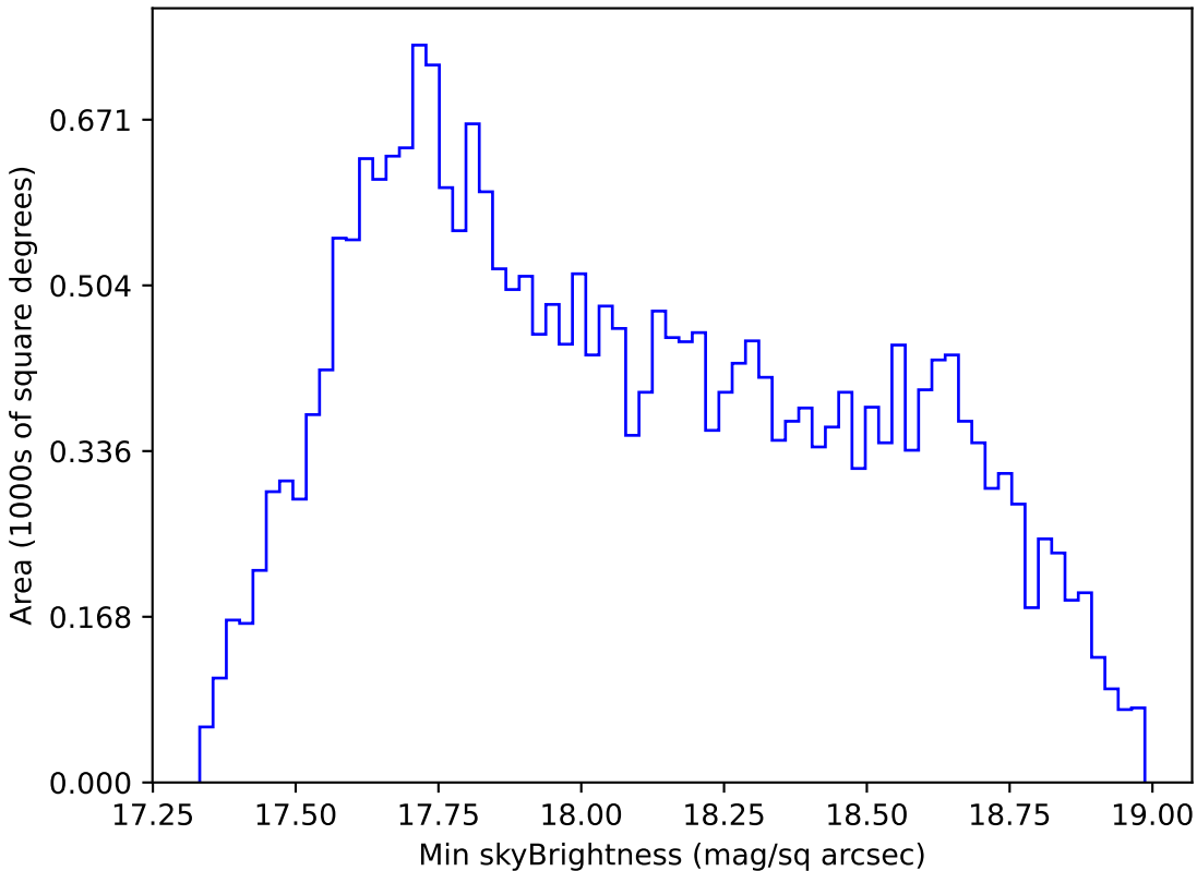
too_elab_r32_d2_giz_v3.4_10yrs All sky i band: Min skyBrightness
