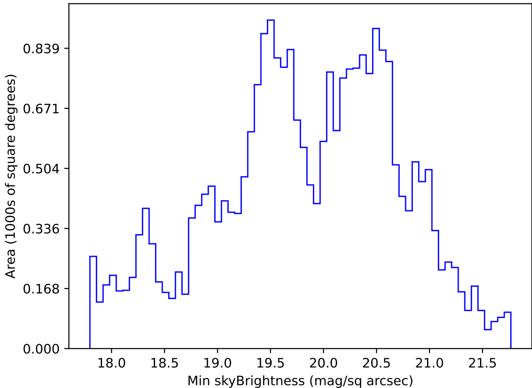
too_elab_r32_d2_giz_v3.4_10yrs All sky g band: Min skyBrightness
