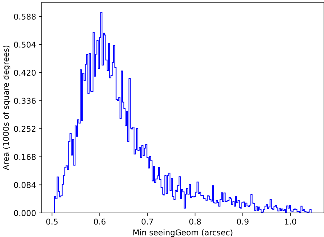
too_elab_r32_d2_giz_v3.4_10yrs Yr 1 z band: Min seeingGeom
