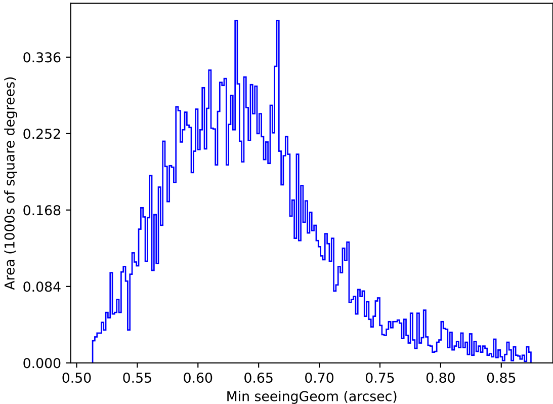
too_elab_r32_d2_giz_v3.4_10yrs Yr 1 y band: Min seeingGeom
