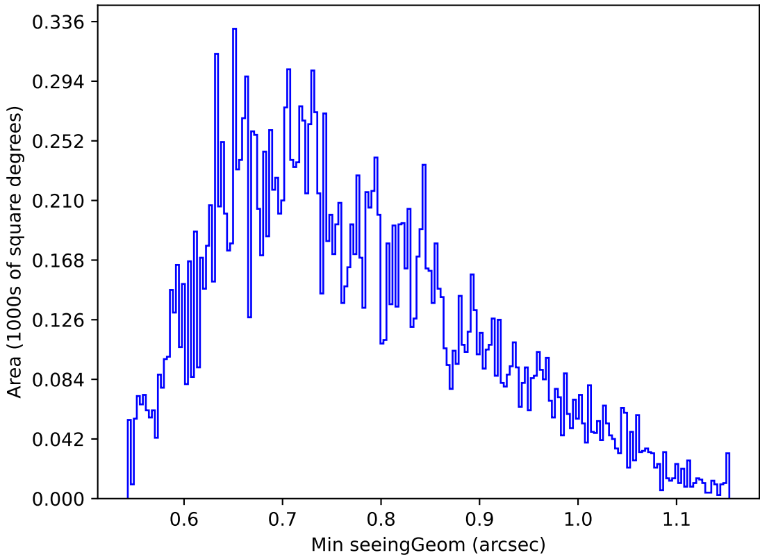
too_elab_r32_d2_giz_v3.4_10yrs Yr 1 u band: Min seeingGeom
