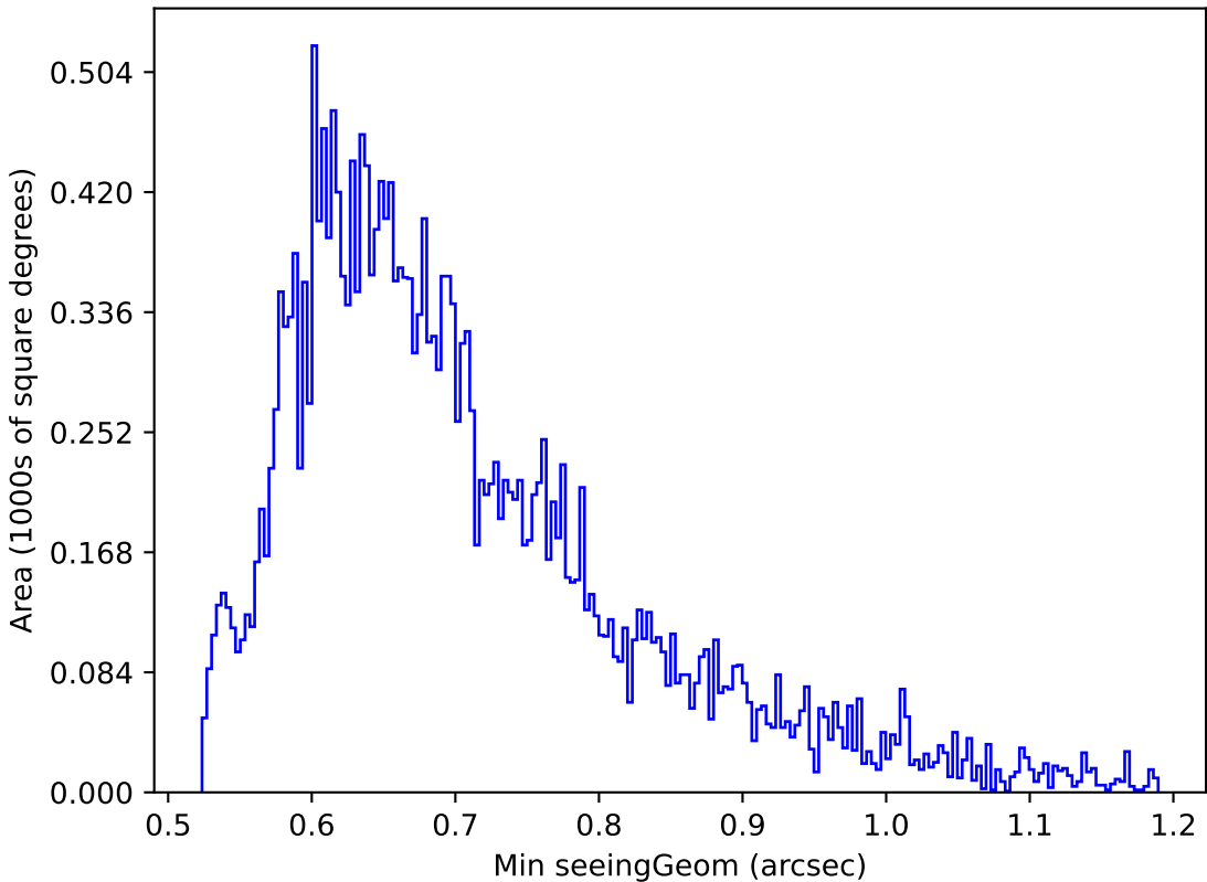
too_elab_r32_d2_giz_v3.4_10yrs Yr 1 g band: Min seeingGeom
