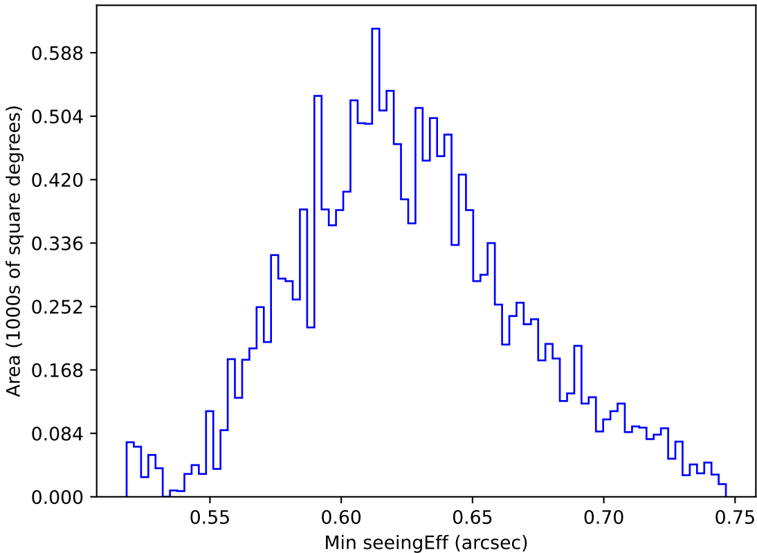
too_elab_r32_d2_giz_v3.4_10yrs WFD y band: Min seeingEff
