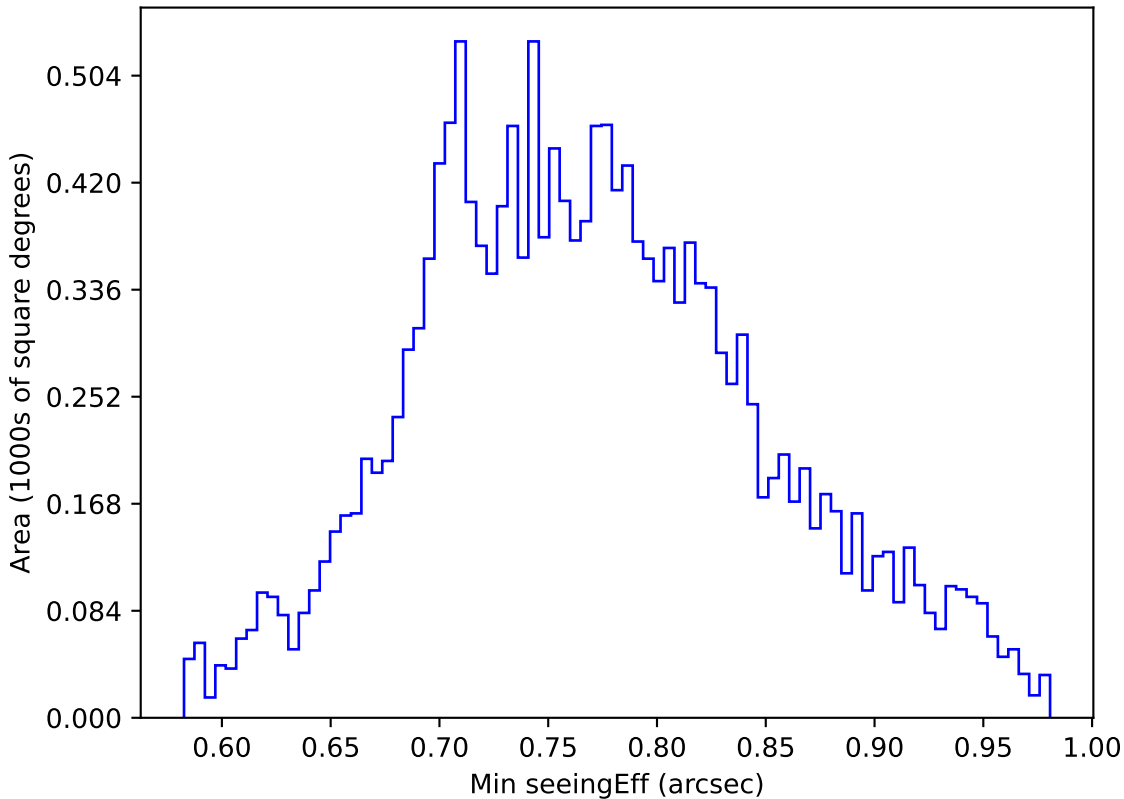
too_elab_r32_d2_giz_v3.4_10yrs WFD u band: Min seeingEff
