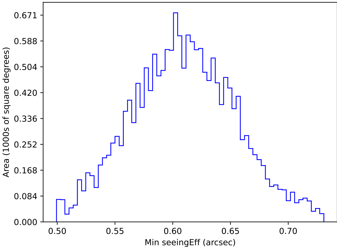
too_elab_r32_d2_giz_v3.4_10yrs WFD r band: Min seeingEff
