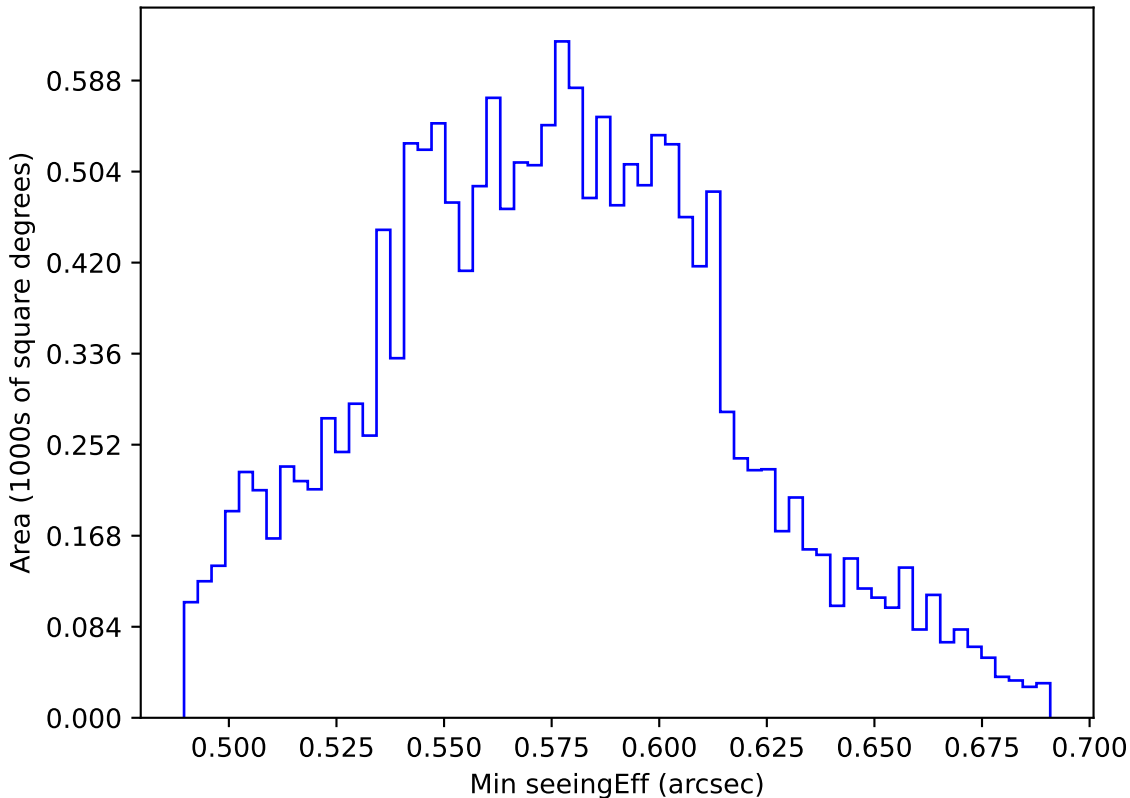
too_elab_r32_d2_giz_v3.4_10yrs WFD all bands: Min seeingEff
