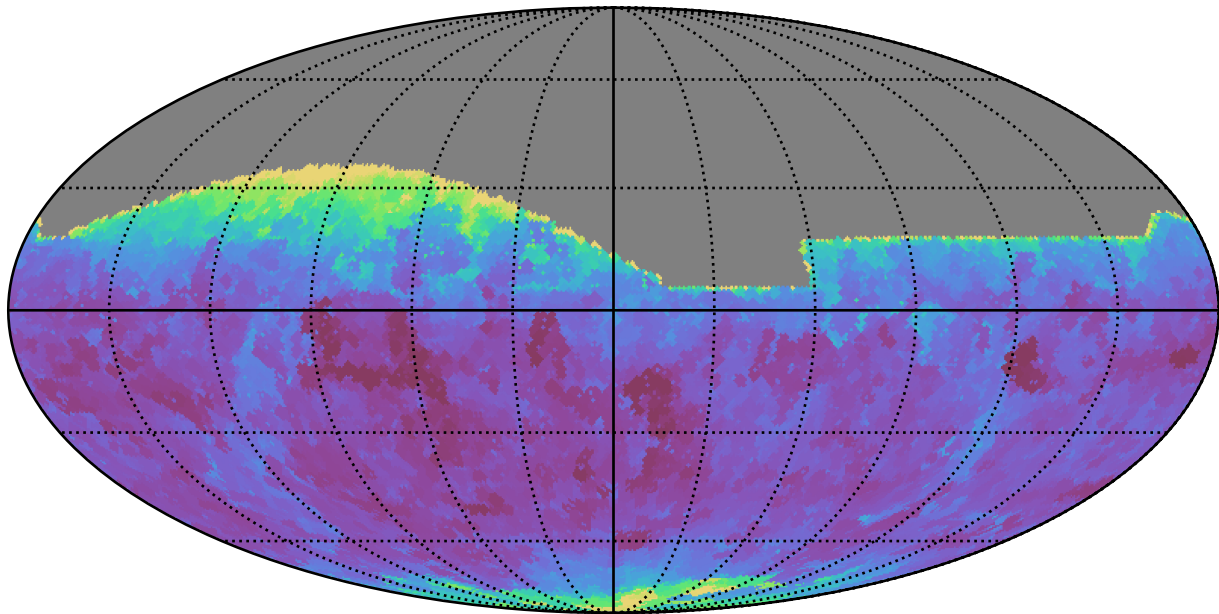
too_elab_r32_d2_giz_v3.4_10yrs All sky z band: Min seeingEff
