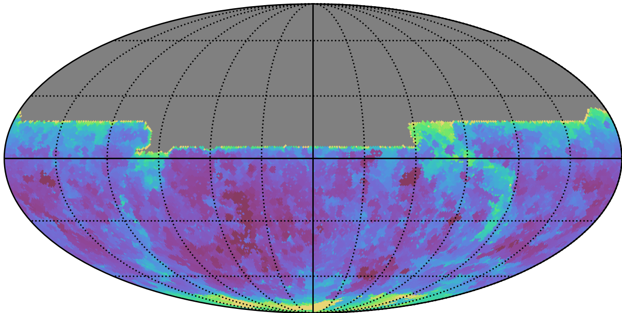
too_elab_r32_d2_giz_v3.4_10yrs All sky y band: Min seeingEff
