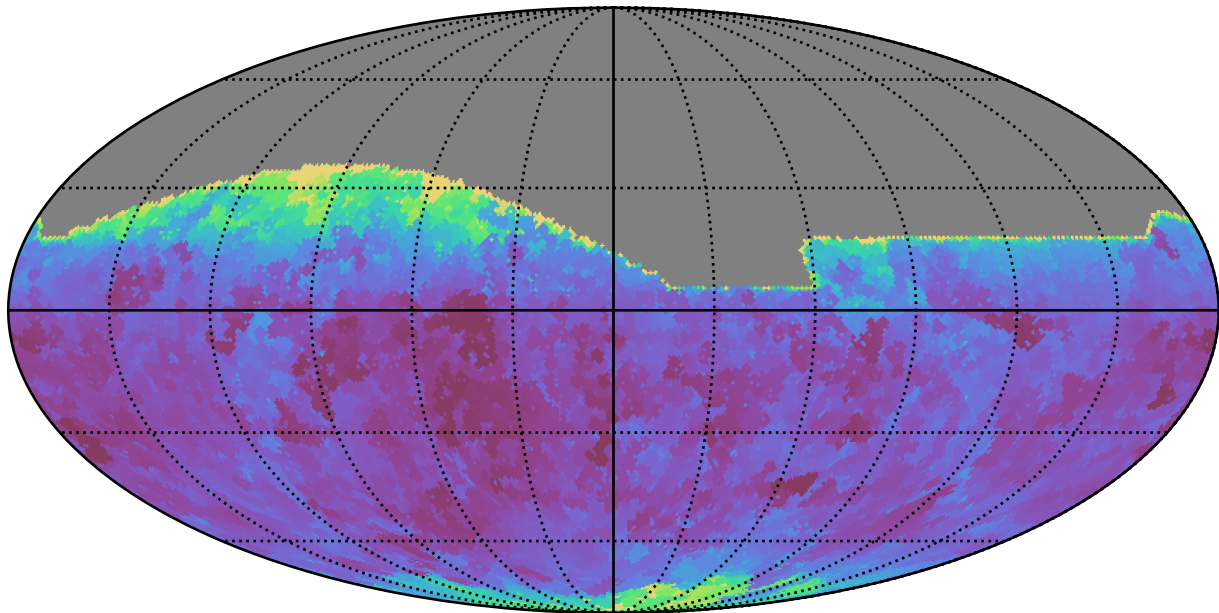
too_elab_r32_d2_giz_v3.4_10yrs All sky r band: Min seeingEff
