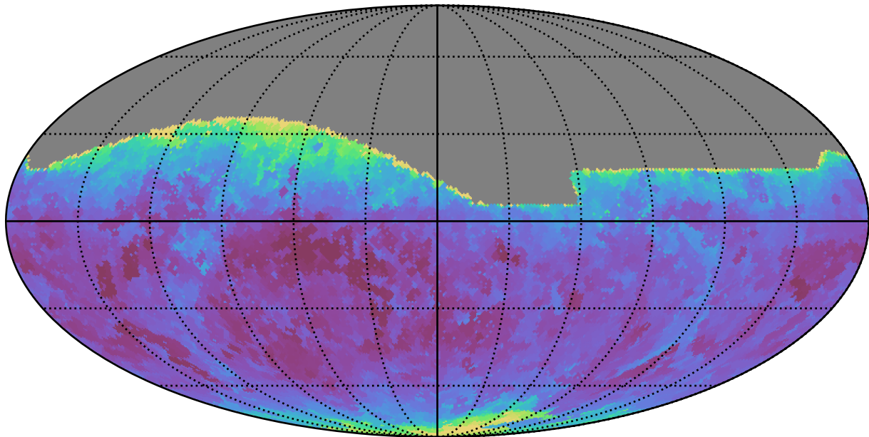
too_elab_r32_d2_giz_v3.4_10yrs All sky i band: Min seeingEff
