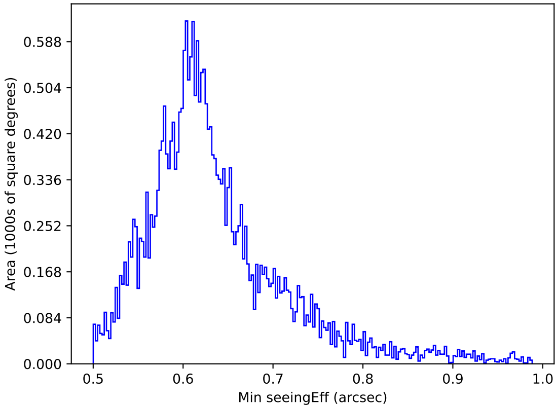
too_elab_r32_d2_giz_v3.4_10yrs All sky i band: Min seeingEff
