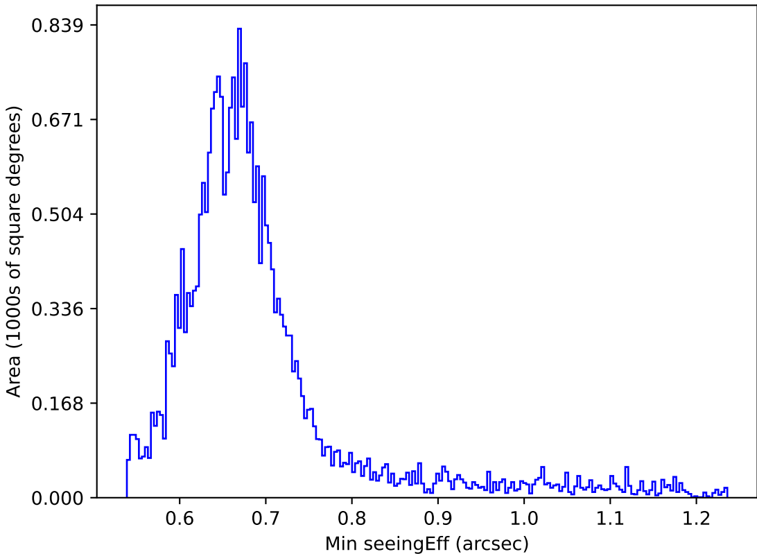
too_elab_r32_d2_giz_v3.4_10yrs All sky g band: Min seeingEff
