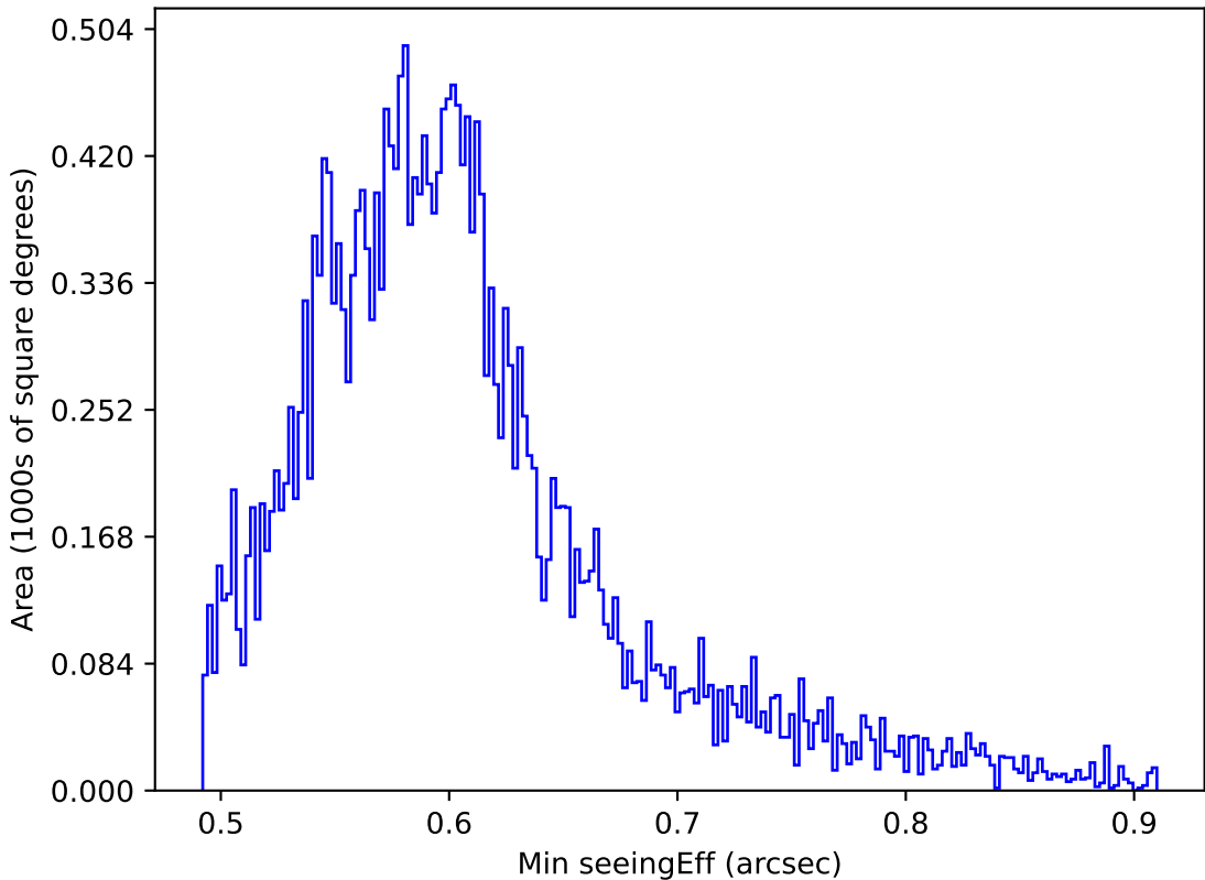
too_elab_r32_d2_giz_v3.4_10yrs All sky all bands: Min seeingEff
