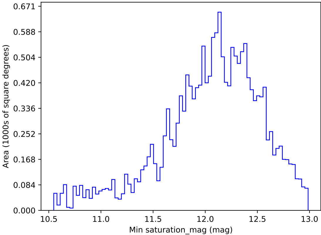
too_elab_r32_d2_giz_v3.4_10yrs WFD z band: Min saturation_mag
