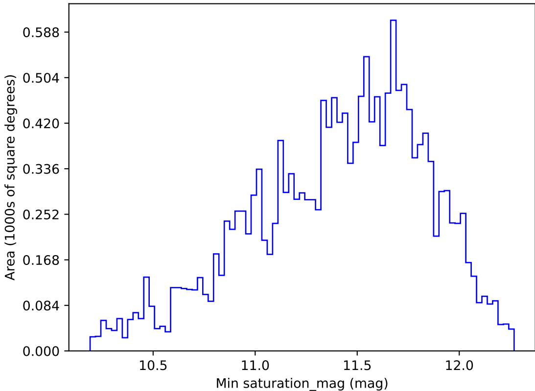
too_elab_r32_d2_giz_v3.4_10yrs WFD u band: Min saturation_mag
