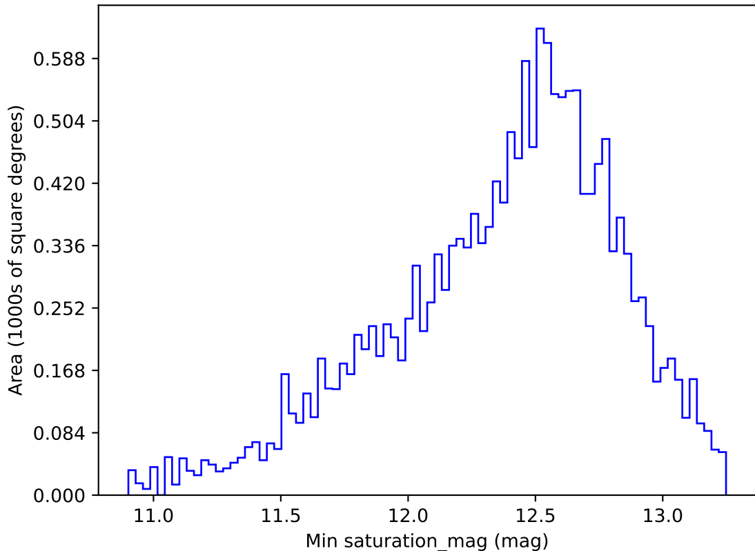
too_elab_r32_d2_giz_v3.4_10yrs WFD i band: Min saturation_mag
