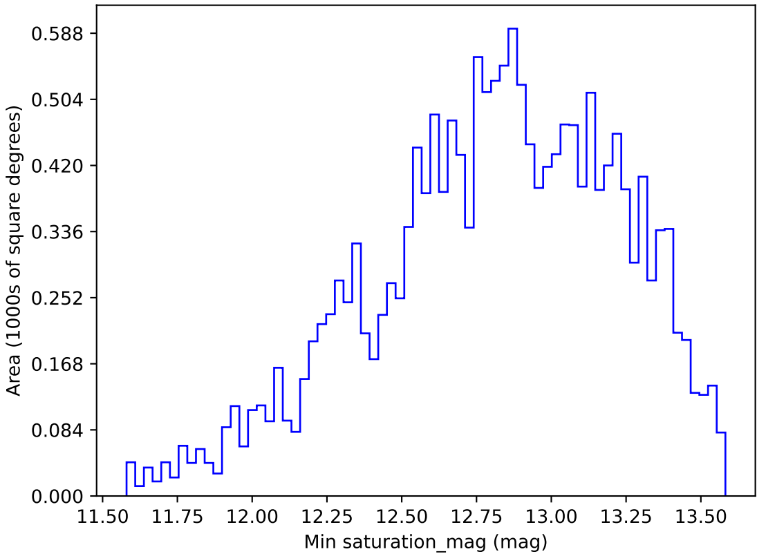
too_elab_r32_d2_giz_v3.4_10yrs WFD g band: Min saturation_mag
