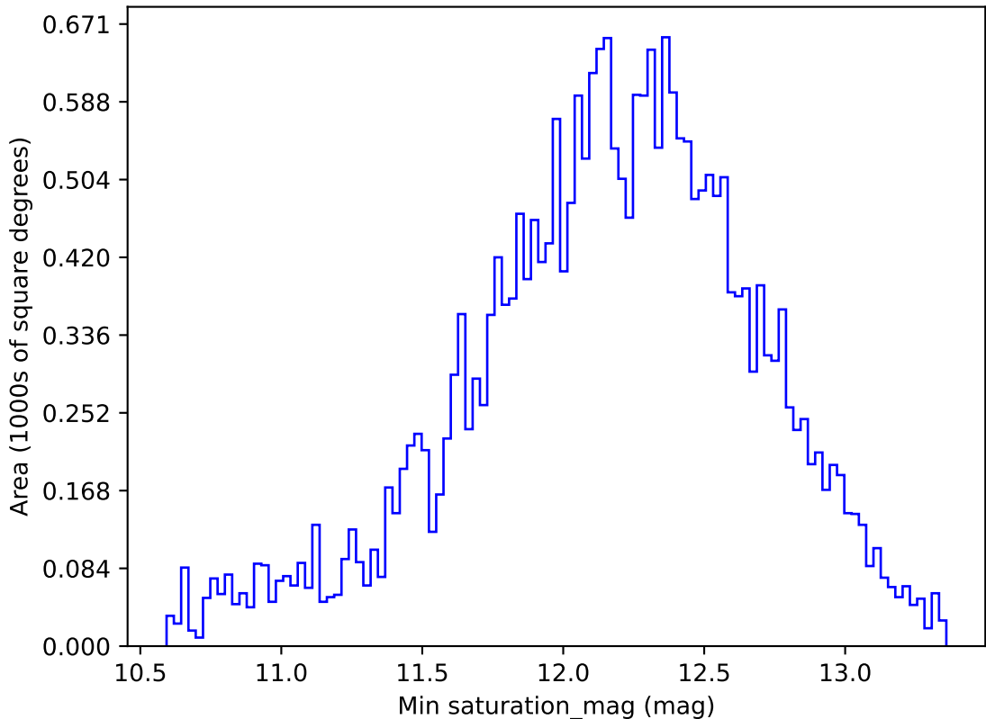
too_elab_r32_d2_giz_v3.4_10yrs All sky z band: Min saturation_mag
