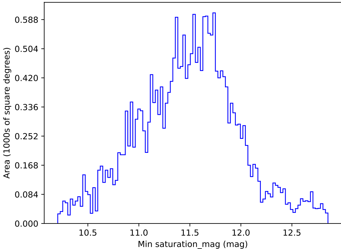
too_elab_r32_d2_giz_v3.4_10yrs All sky u band: Min saturation_mag
