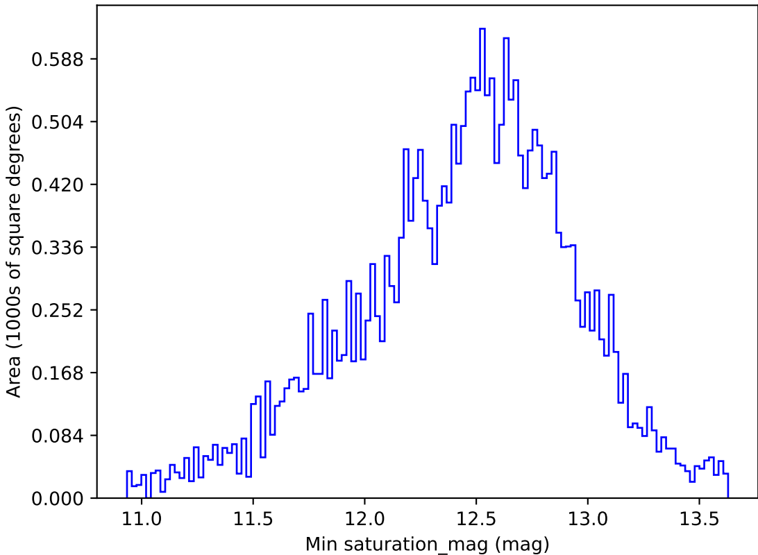
too_elab_r32_d2_giz_v3.4_10yrs All sky i band: Min saturation_mag
