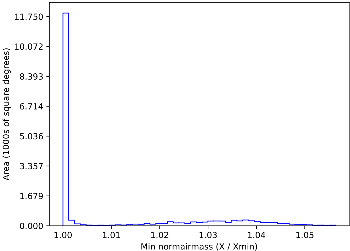
too_elab_r32_d2_giz_v3.4_10yrs WFD u band: Min normairmass
