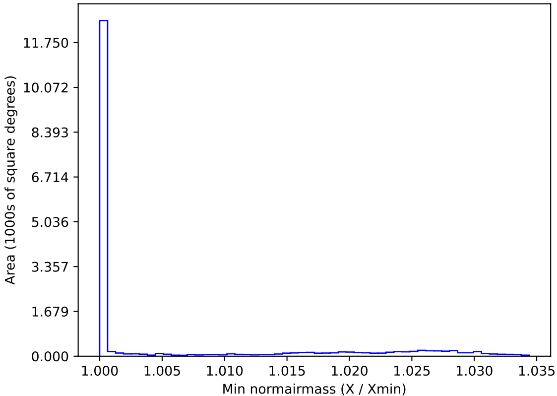
too_elab_r32_d2_giz_v3.4_10yrs WFD i band: Min normairmass
