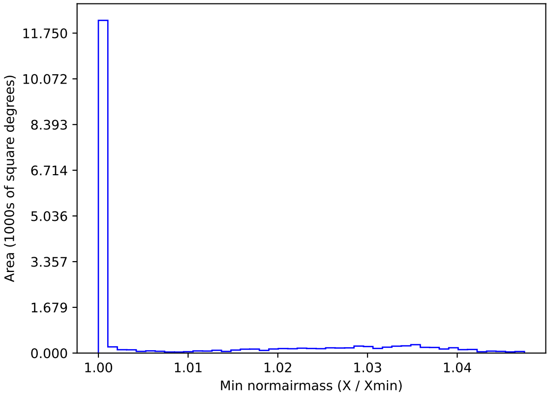
too_elab_r32_d2_giz_v3.4_10yrs WFD g band: Min normairmass
