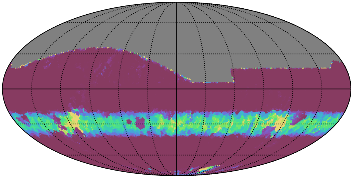
too_elab_r32_d2_giz_v3.4_10yrs All sky z band: Min normairmass
