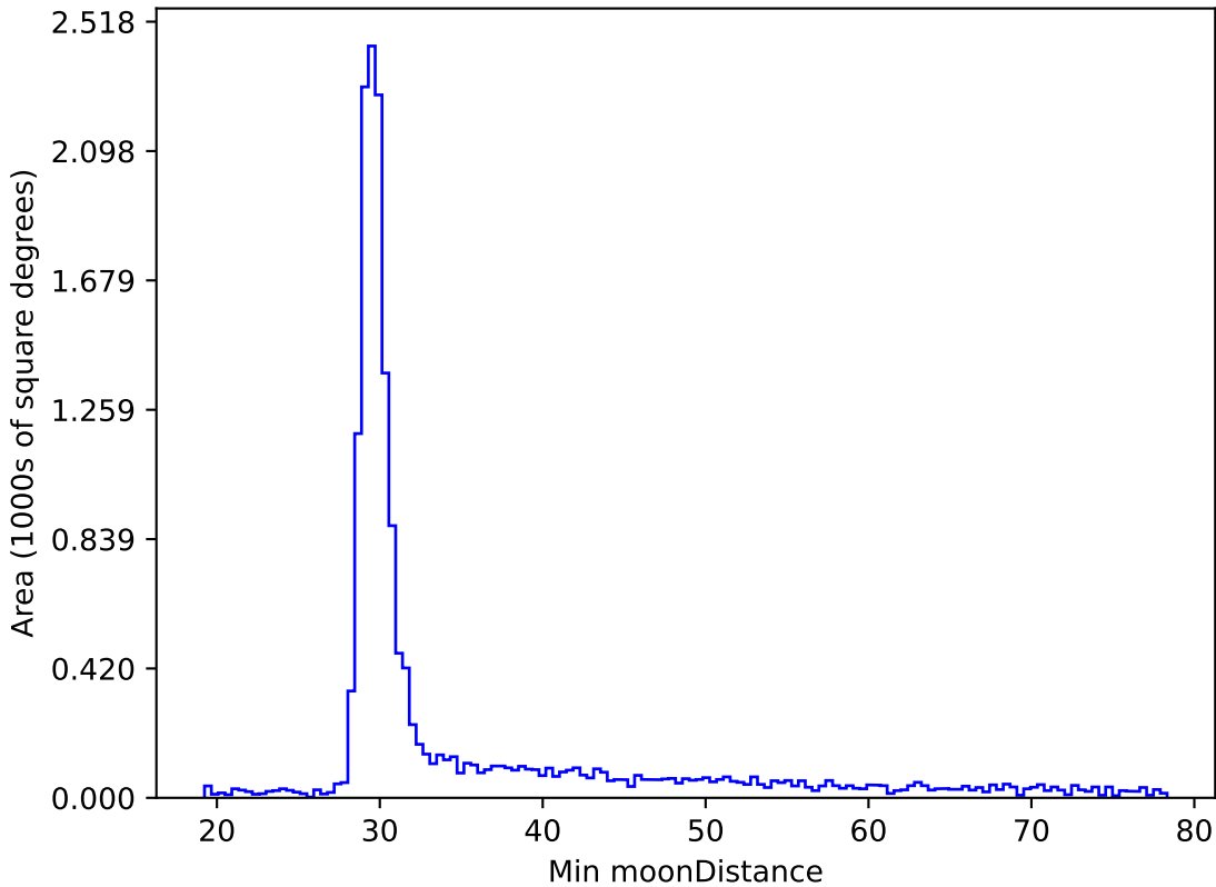
too_elab_r32_d2_giz_v3.4_10yrs WFD z band: Min moonDistance
