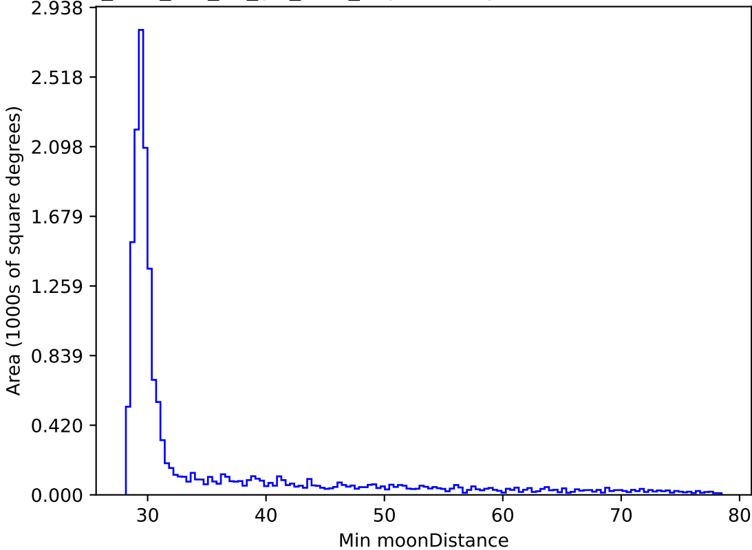
too_elab_r32_d2_giz_v3.4_10yrs WFD y band: Min moonDistance
