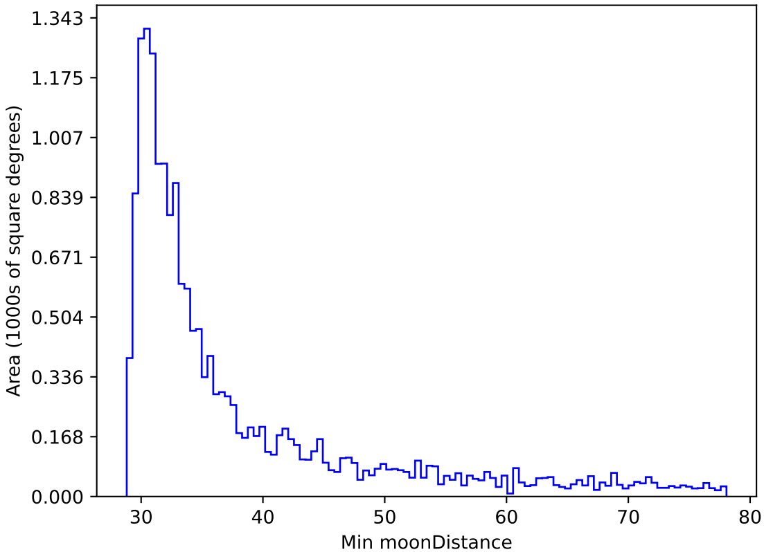
too_elab_r32_d2_giz_v3.4_10yrs WFD r band: Min moonDistance
