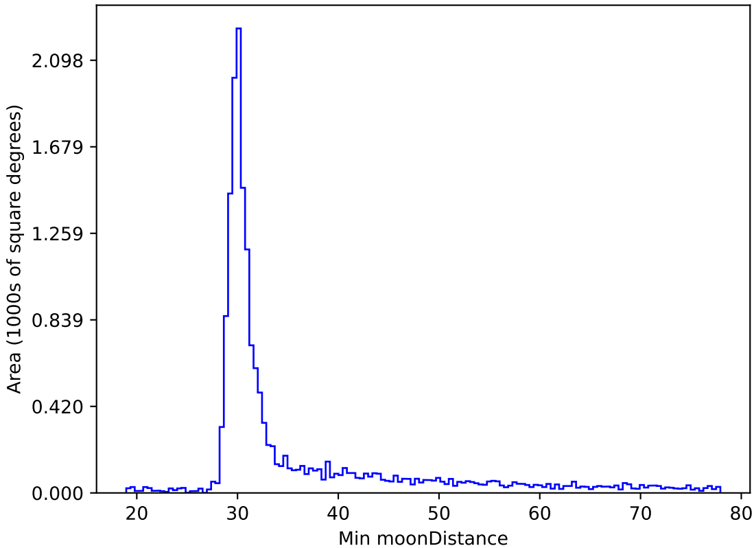
too_elab_r32_d2_giz_v3.4_10yrs WFD i band: Min moonDistance
